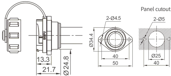
2-hole flange Mate with SY2520, SY2124
