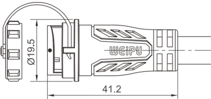
Single-Ended Cordsets--Receptacle Mate with SY1320, SY1324
