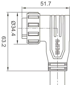
Single-Ended Cordsets--Plug Mate with SY2521, SY2512, SY2513, SY2515
