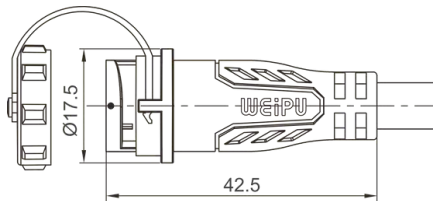
Single-Ended Cordsets--Receptacle Mate with SY1120, SY1124
