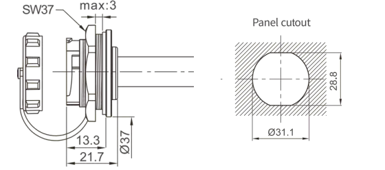
Front-nut mount Mate with SY2120,SY2124
