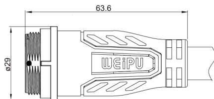
Single-Ended Cordsets--Receptacle Mate with SP2120,SP2124
