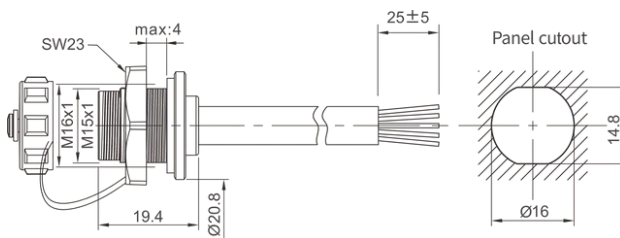
Front-nut mount Matewith SP1320,SP1324
