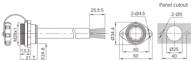
2-hole flange Mate with SP2520,SP2524
