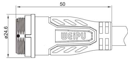
Single-Ended Cordsets--Receptacle Mate with SP1720,SP1724
