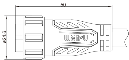
Single-Ended Cordsets--Plug Matewith SP1721,SP1712
