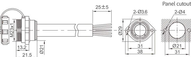
2-hole flange Mate with SP2120,SP2124
