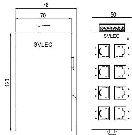
EST280 8 port ethernet switch
