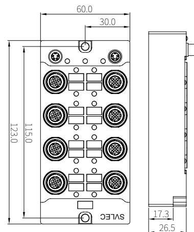
ESP180 8 port ethernet switch IP67
