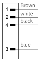
4-core single ended
