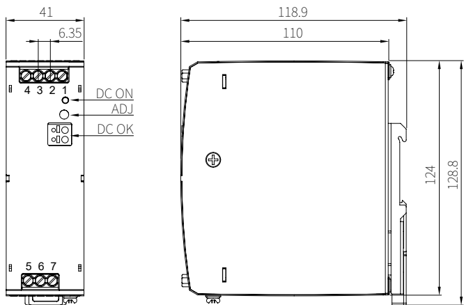
PR-240-24 Drawing
