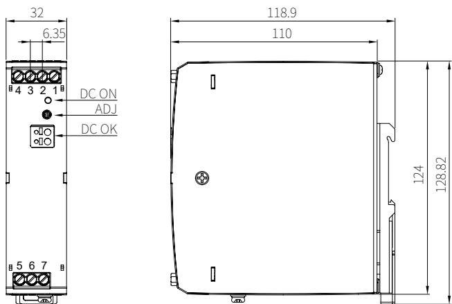
PR-120-24 Drawing
