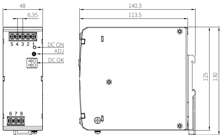
PR-480-24/48 Drawing
