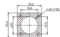
Female contact angled square flange receptacle
